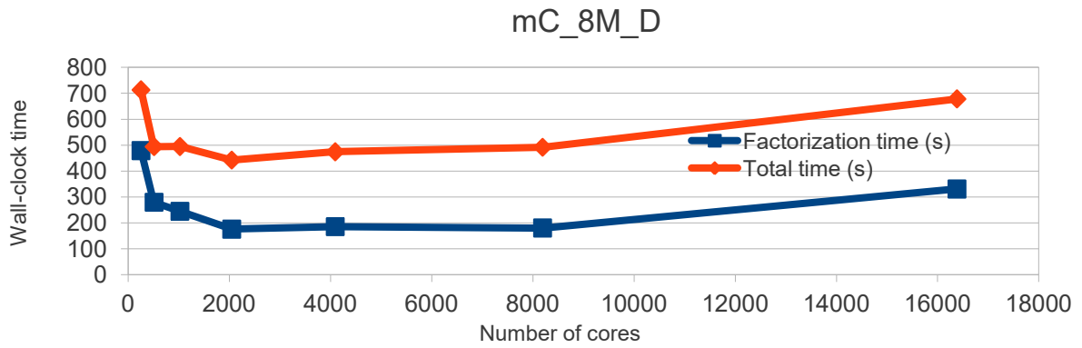
Fig. 5. The performance of SuperLU_MCDT for mC_8M_D
