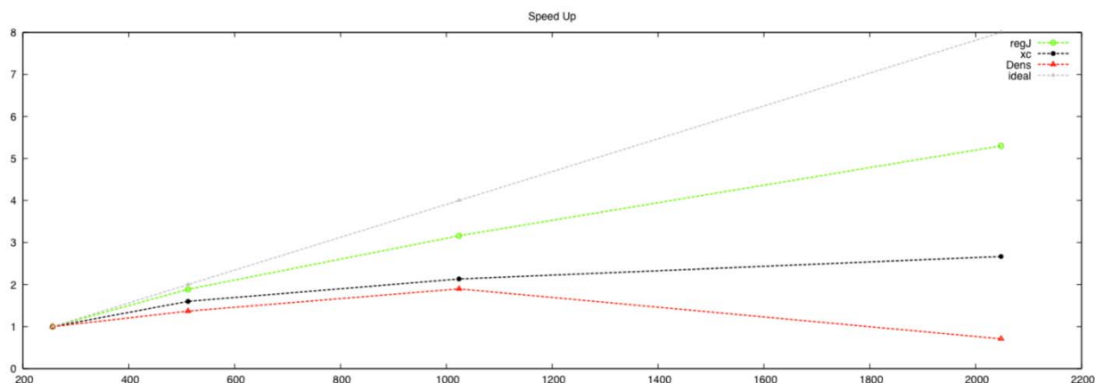
Figure 7: Hybrid MPI/OpenMP speed-up relative to the 32/8 reference for insulin using BLYP/cc-pVDZ
