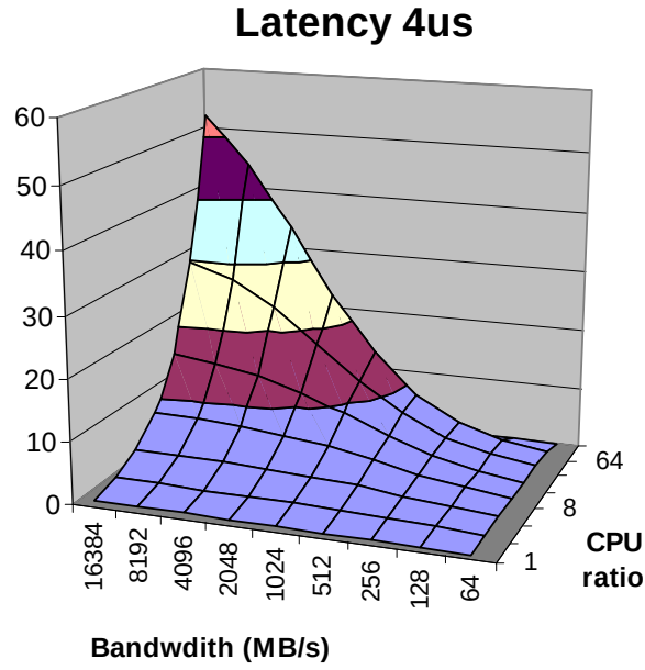
Figure 9: Fixed latency of 4 microseconds at the variations of 2 parameters keeping the third one constant
