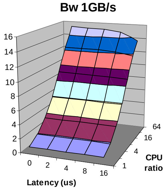
Figure 11: The scenario with a fixed bandwidth of 1GB/s that is quite similar to the current bandwidth on the machine used to obtain the trace file
