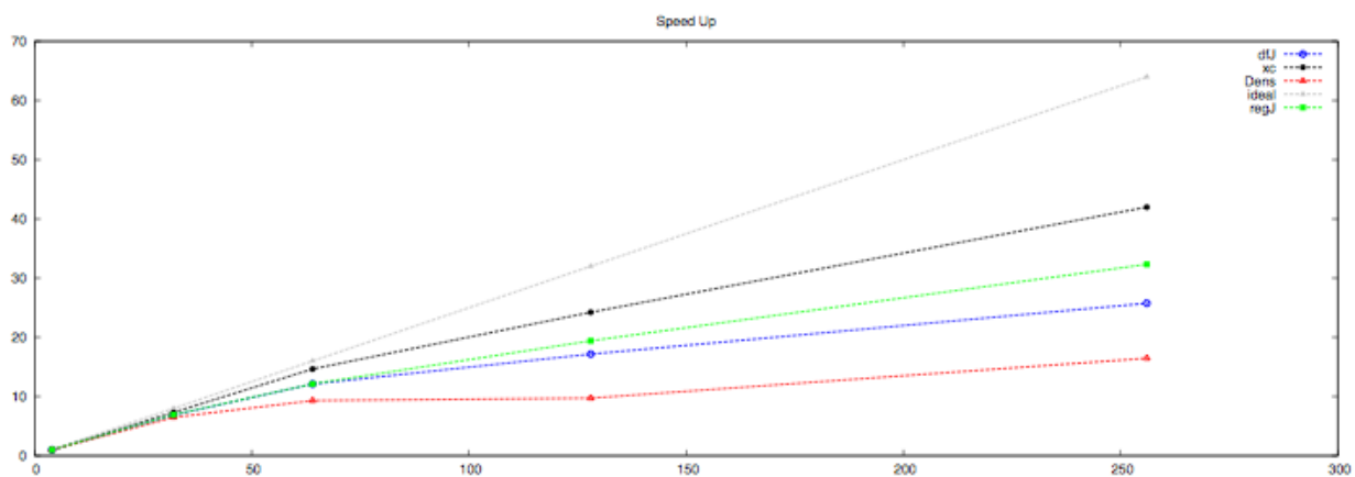
Figure 4: Pure MPI speed-up relative to the MPI/OMP 4/1 reference for valinomycin using BLYP/aug-cc-pVDZ (df-def2)
