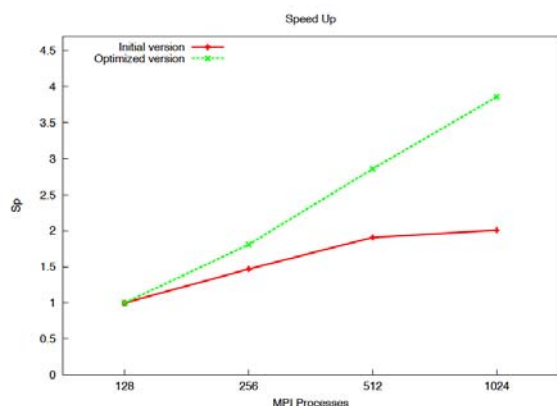
Figure 2: Speedup after optimization and redesign
