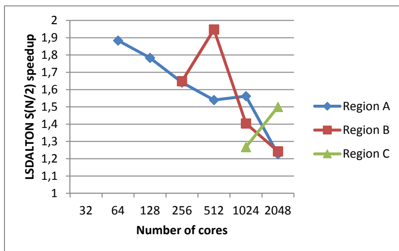
Figure 8: LSDALTON S(N/2) parallel scaling for QM regions A, B and C. Ideal scaling is equivalent to S(N/2)=2 .
