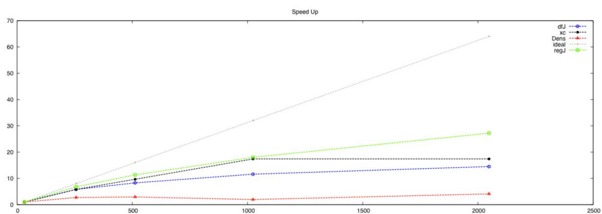
Figure 5: Hybrid MPI/OpenMP speed-up relative to the 4/8 reference for valinomycin using BLYP/aug-cc-pVDZ (df-def2)
