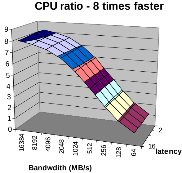
Figure 10: The impact of improving the computing time with no changes on the network requirements
