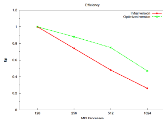
Figure 3: Parallel efficiency after optimization and redesign
